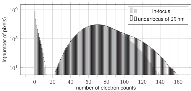
Fig. 8. Effect of focus on dynamic range. Distribution of electron counts for the full simulated 4D-STEM scan for 300 kV using an in-focus setting and an under-focus of 25 nm. The first peak of both distributions shows the dark field counts and the second, broader peak the bright field counts.
